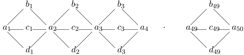
Figure 4: Double diamond equalities
